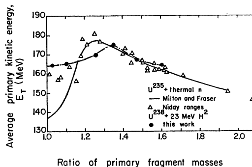
Fig. 4. Average total kinetic energy before neutron emission vs primary mass ratio. Symbols are as follows: U 235 +thermal n, solid line from reference 12, open triangles from range data of reference 9 and \nu values from curve A of Fig. 1; U 236 +23-MeV H 2 , closed circles and dot-dash line, range data from this work and all \nu values taken as 3.0. Ranges taken as proportional to E^{2/3} .
